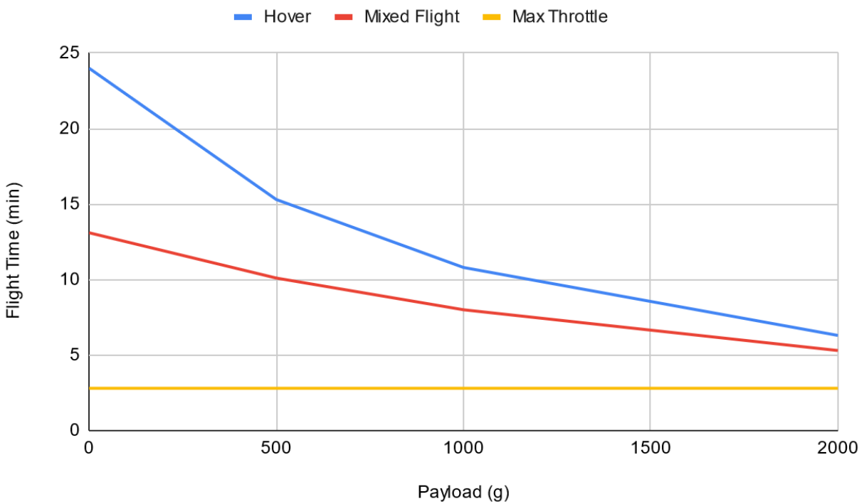
Figure 1: Graph showing payload vs flight time for hovering, mixed flight, and maximum throttle
